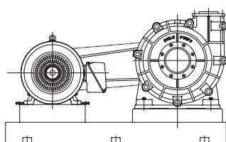
HORIZONTAL V-BELT DRIVE ( HR )
